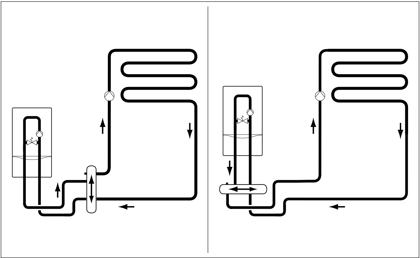
WH 40 (306720)
